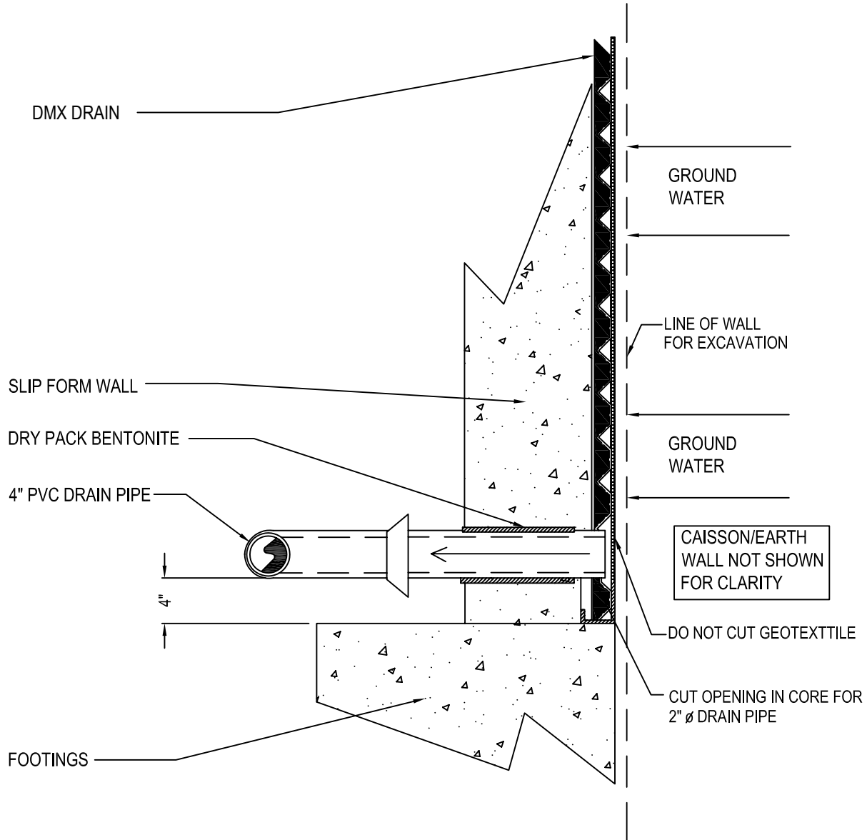
DETAIL 'A'
