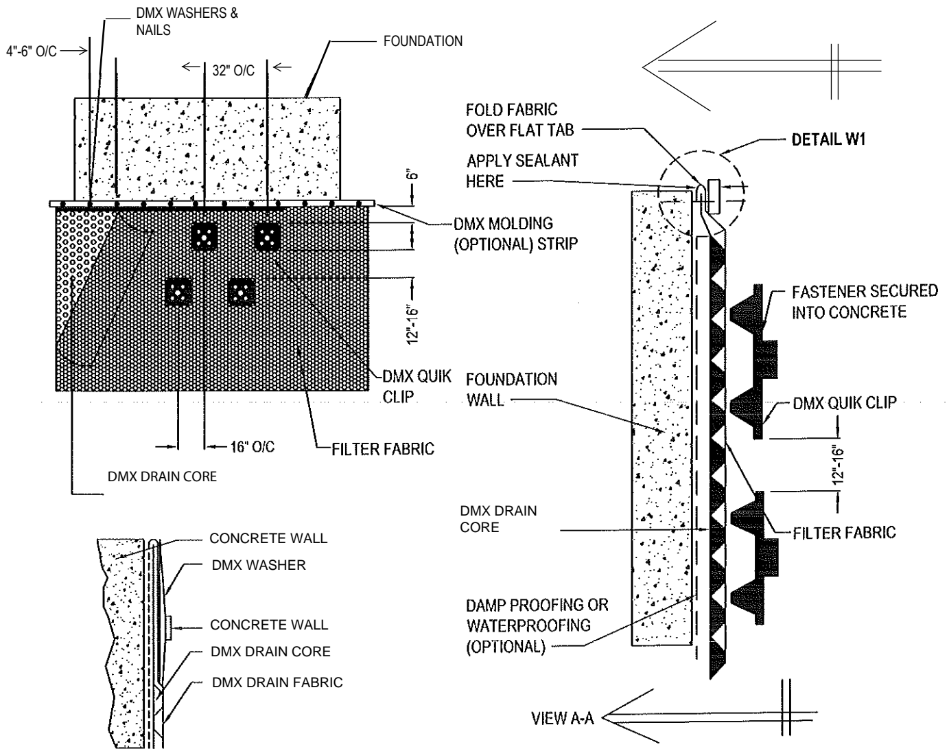
DETAIL W1
