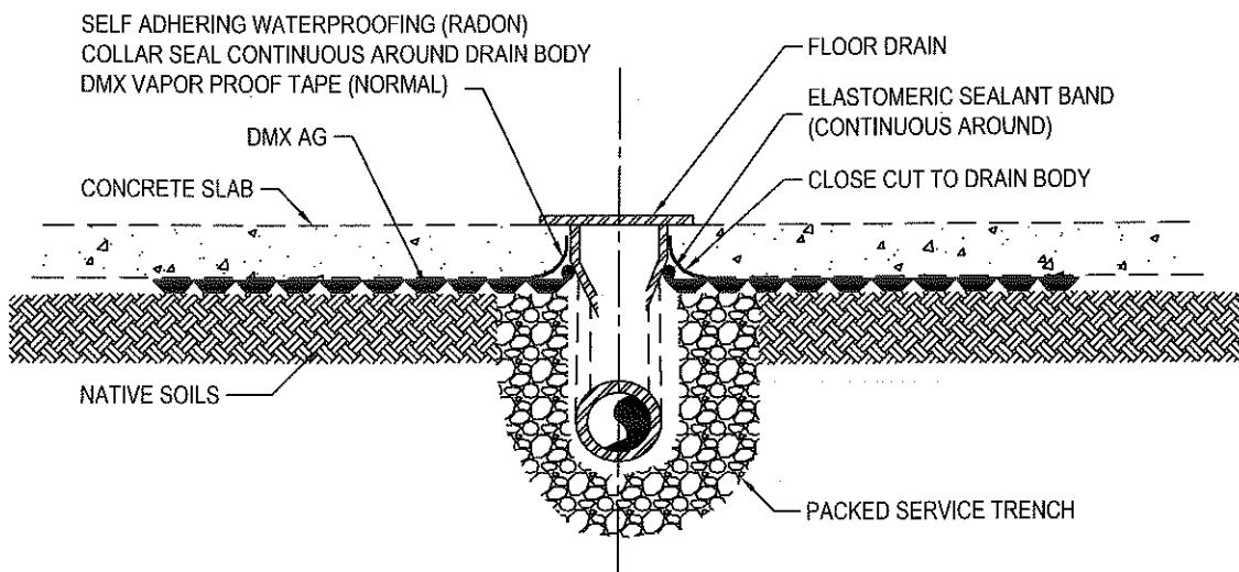
SEAL AROUND FLOOR DRAIN PENETRATIONS - TYPICAL
