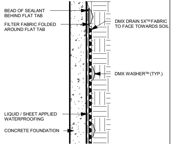
DMX DRAIN 5X™ ON CONCRETE FOUNDATION (SECTION VIEW - N.T.S)
