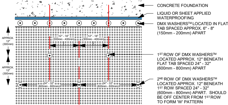
DMX DRAIN 5X™ ON CONCRETE FOUNDATION (FRONT VIEW - 1:20)
