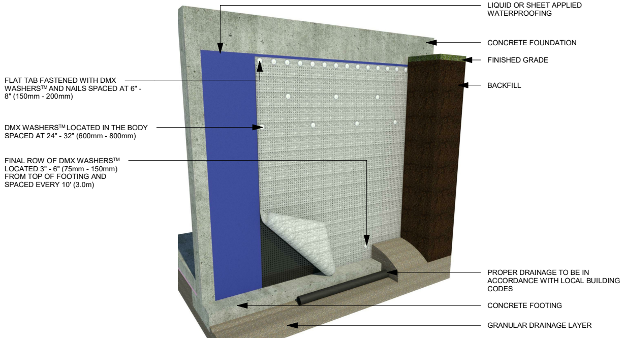
DMX DRAIN 5X™ ON CONCRETE FOUNDATION (ISO)
