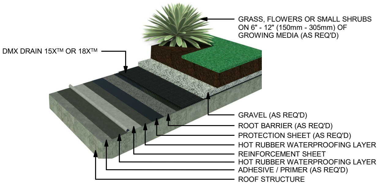
SEMI-INTENSIVE GREEN ROOF ON DMX DRAIN (ISO)
