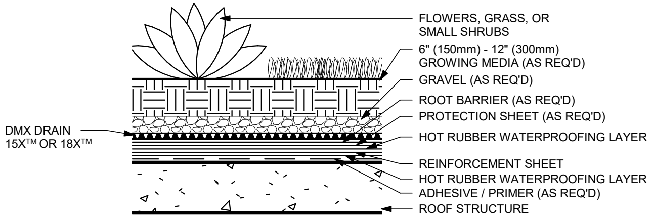
SEMI-INTENSIVE GREEN ROOF ON DMX DRAIN (SECTION VIEW - N.T.S)
