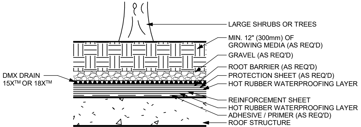
INTENSIVE GREEN ROOF ON DMX DRAIN (SECTION VIEW - N.T.S)
