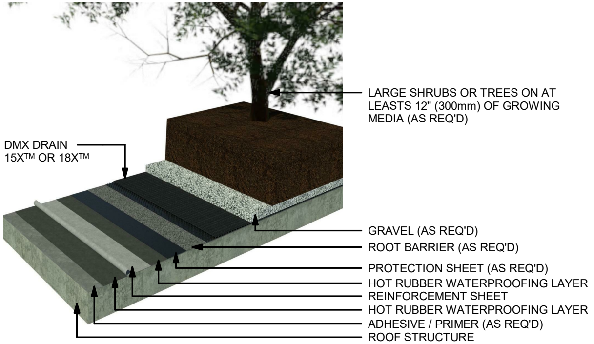
INTENSIVE GREEN ROOF ON DMX DRAIN (ISO)
