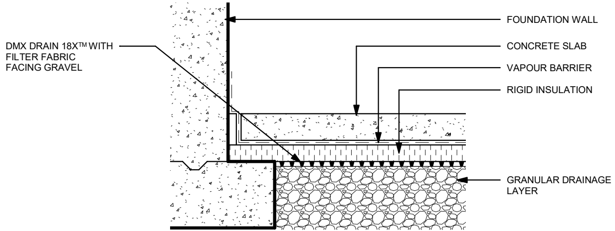
INSULATED CONCRETE SLAB OVER DMX DRAIN 18X™ (SECTION VIEW - N.T.S)
