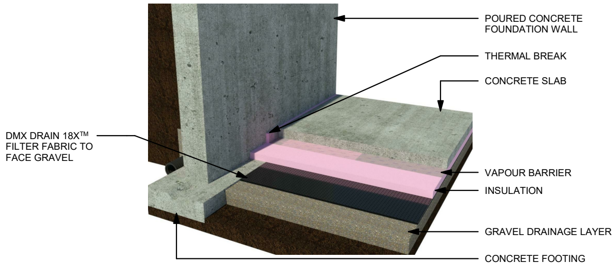
INSULATED CONCRETE SLAB OVER DMX DRAIN 18X™ (ISO)
