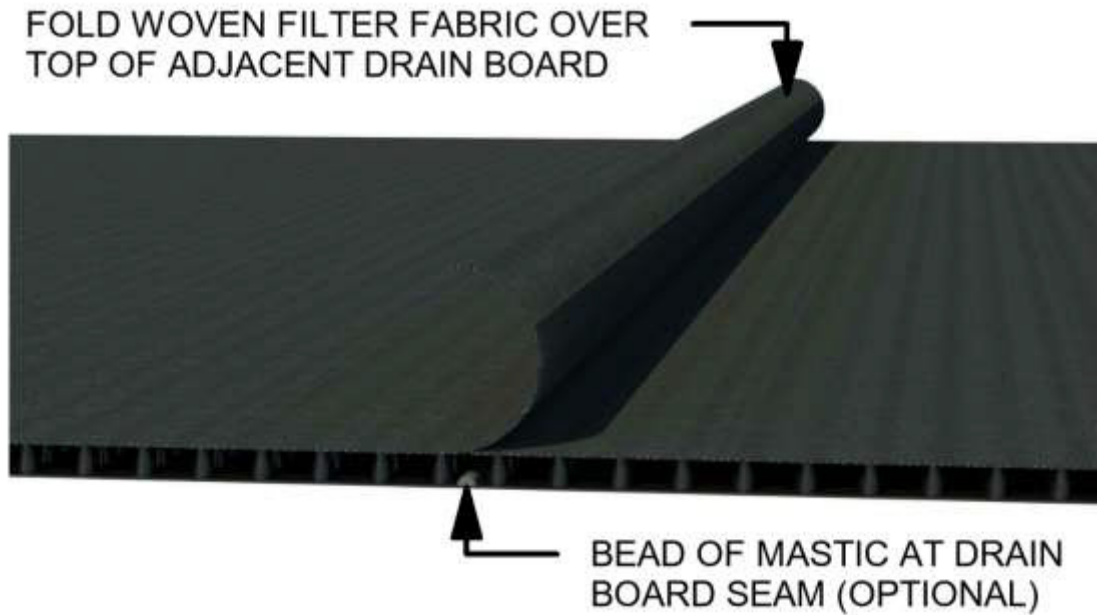
Figure 3 Joining Rolls Step 2
