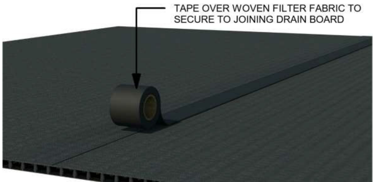
Figure 4 Joining Rolls Step 3 (optional)
