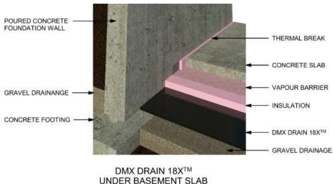
Figure 19 DMX Drain 18X™ Under Basement Slab
