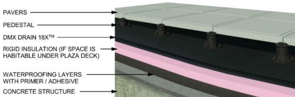
Figure 13 Pedestals on DMX Drain 18X™
