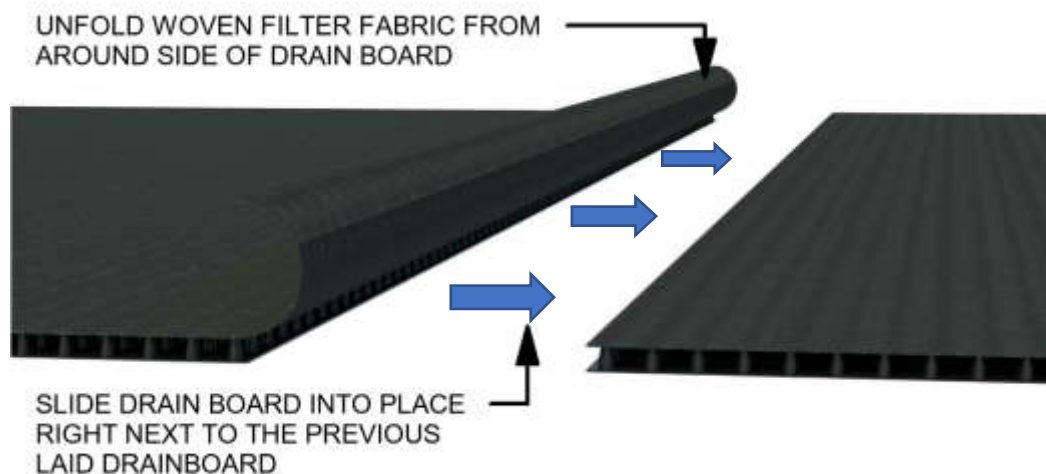
Figure 2 Joining Rolls Step 1
