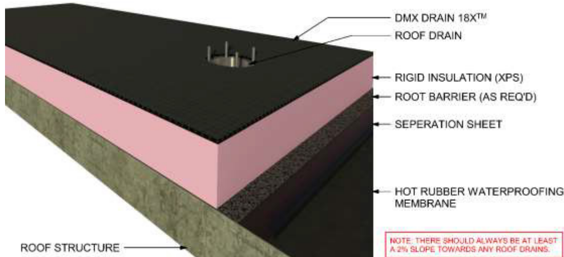
Figure 10 Around Roof Drain Step 3
