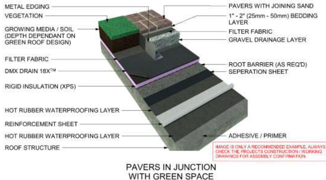
Figure 16 Pavers in Junction with Green Roof
