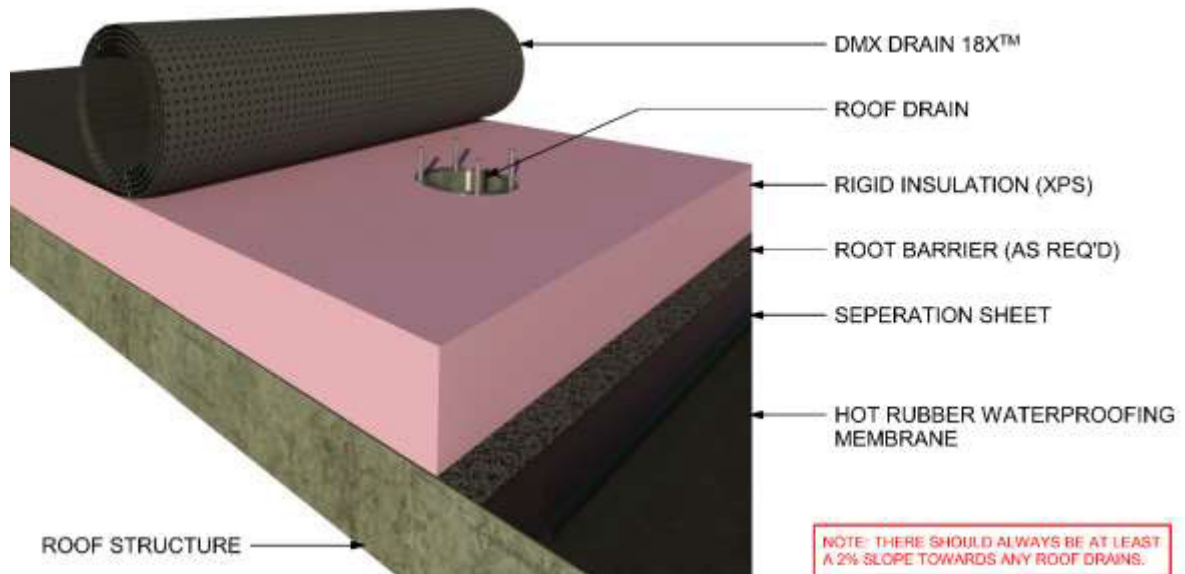
Figure 8 Around Roof Drain Step 1
