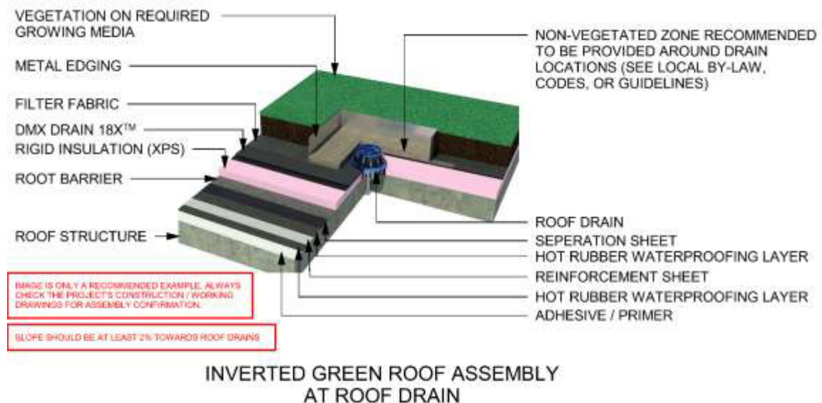
Figure 11 Vegetation Free Zone at Roof Drain
