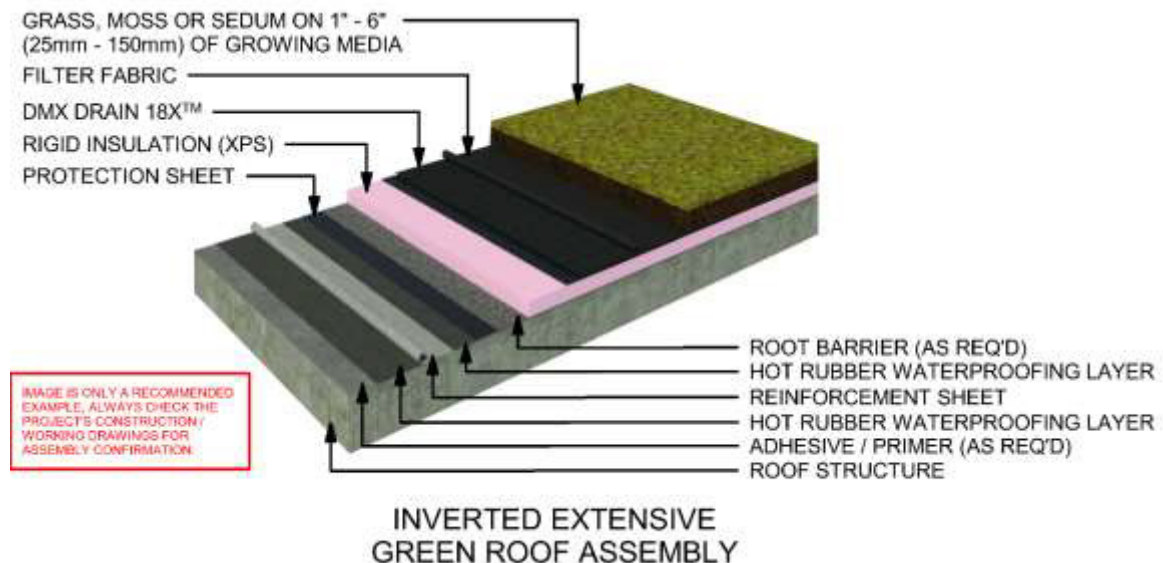
Figure 5 Inverted Extensive Green Roof Assembly
