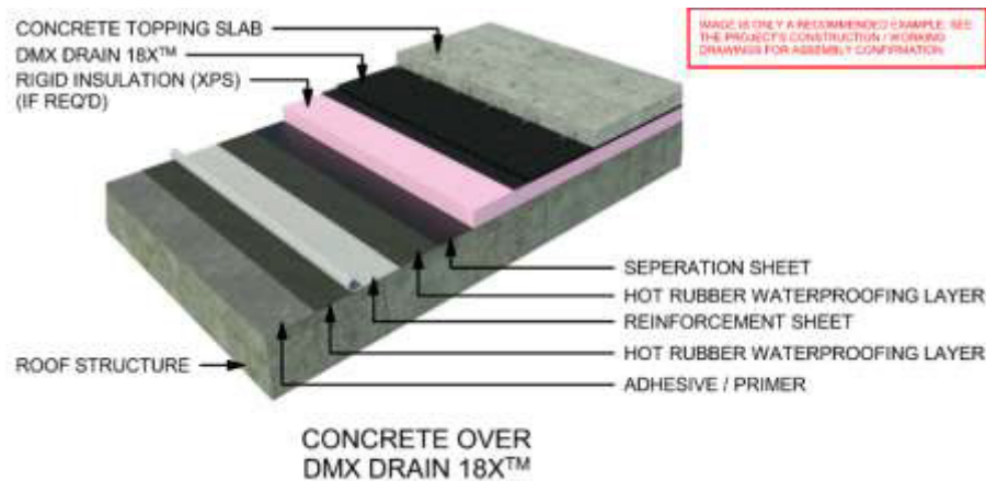
Figure 17 Concrete Over DMX Drain 18X™
