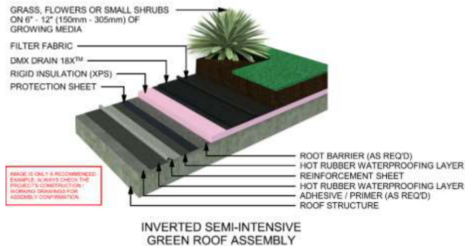
Figure 6 Inverted Semi-Intensive Green Roof Assembly
