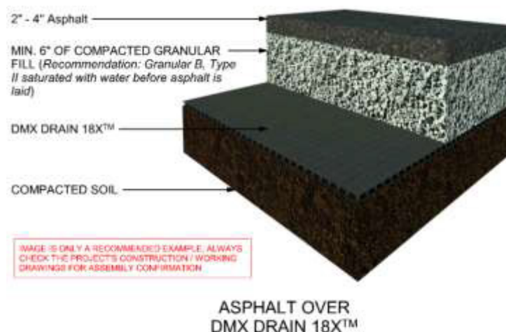
Figure 18 Asphalt Over DMX Drain 18X™
