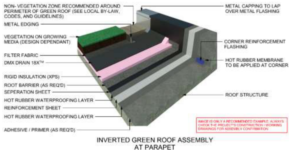
Figure 12 Inverted Green Roof Assembly At Parapet
