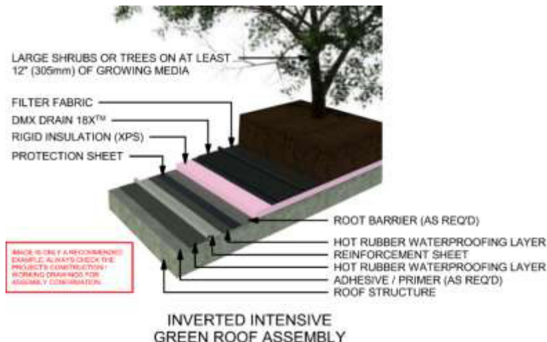
Figure 7 Inverted Intensive Green Roof Assembly
