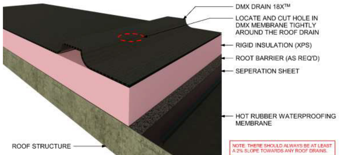
Figure 9 Around Roof Drain Step 2
